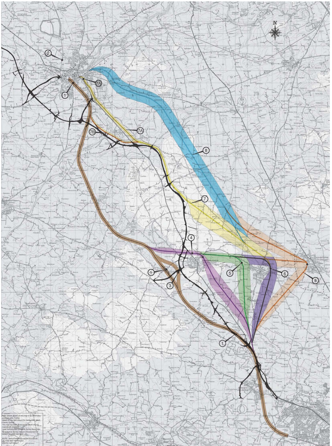
Figure 1: Navan Line Re-opening, Routes Considered at Scoping Stage (2008)
