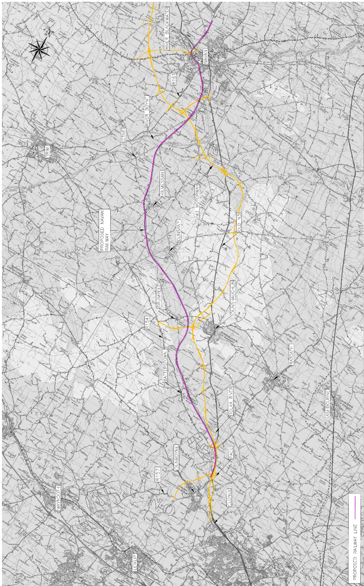
Figure 3: Navan Line Re-opening, Preferred Route (2010)
