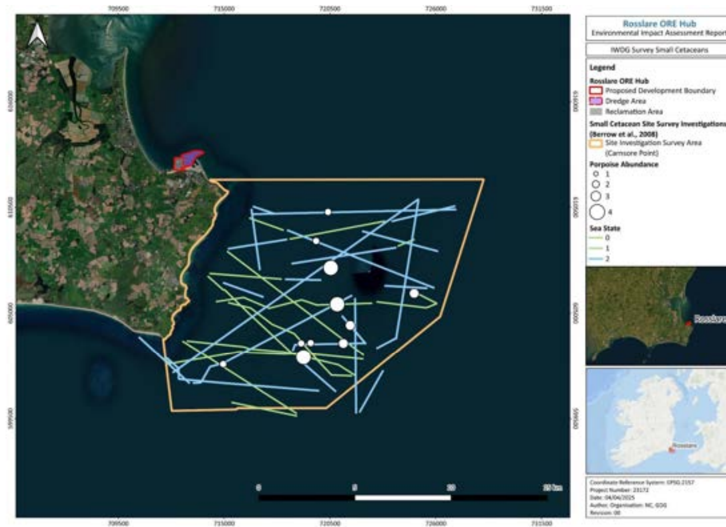
Figure 13-16: Dedicated Harbour Porpoise transects and sightings off Carnsore Point, July to September 2008 (adapted from Berrow et al. , 2008)
