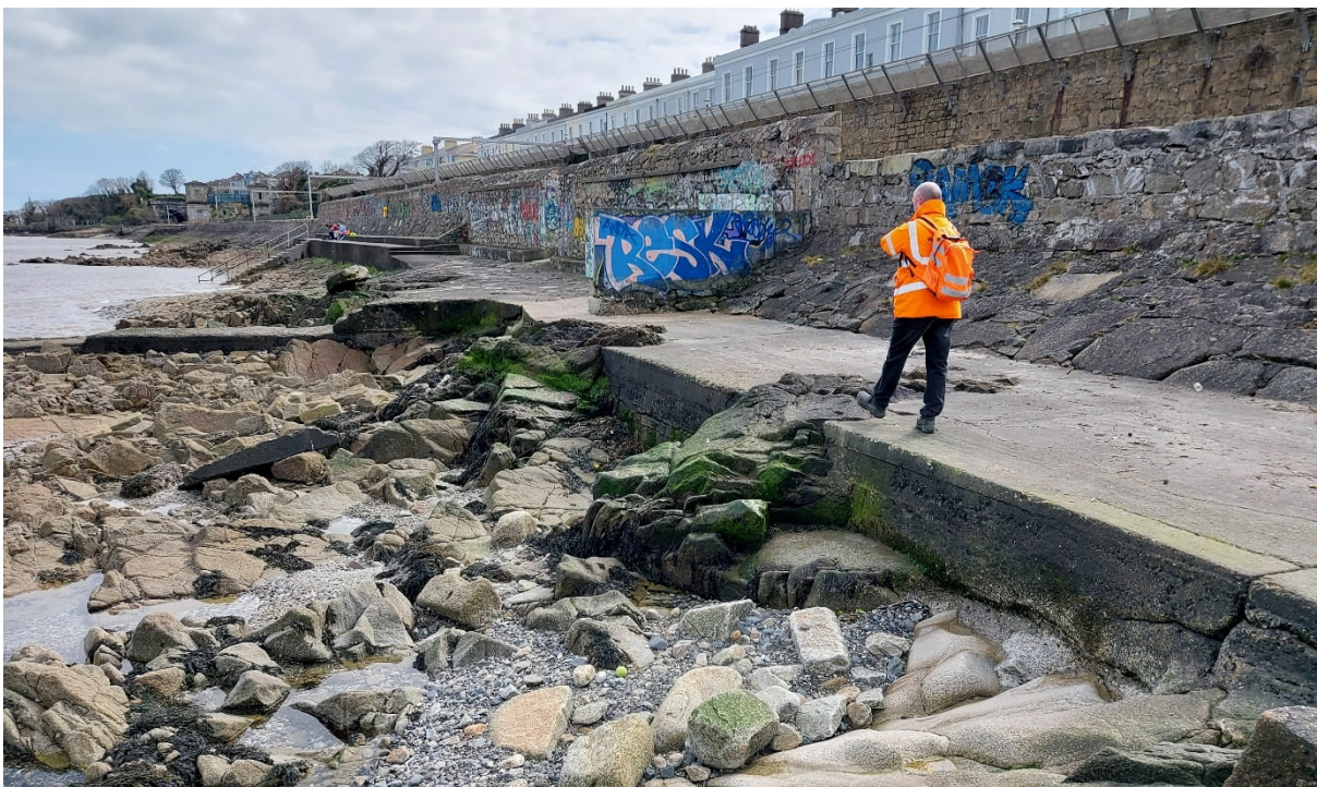
Figure 6 - CCA1-D: The sub-cell's defended section is protected by a masonry revetment and an upstand wall. A concrete walkway has been added along the defences. The foreshore is mainly rocky.
