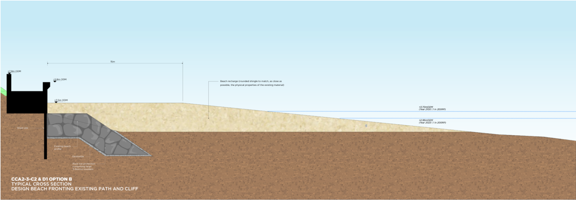
Figure 5-5 CCA2/3-D1 Option B Typical cross section
