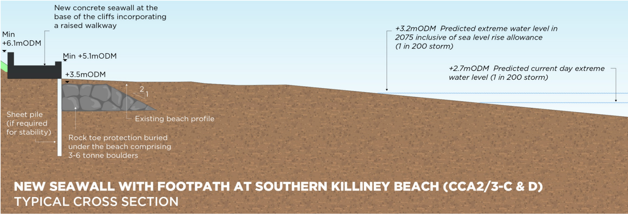
Figure 5-9 CCA2/3 Emerging Preferred Scheme Section at Killiney
