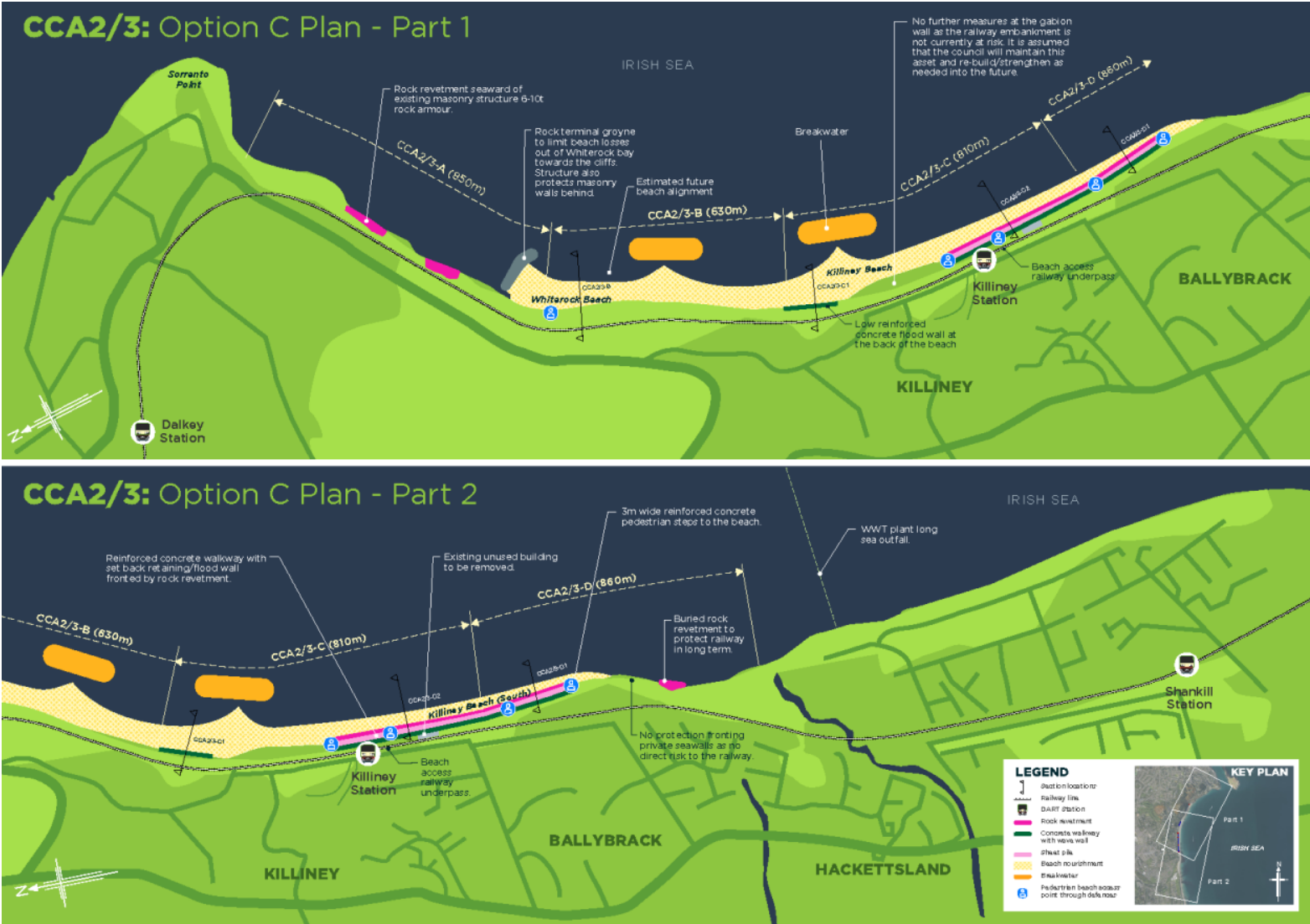
Figure 5-6 CCA2/3 Option C Concept Design Plan
