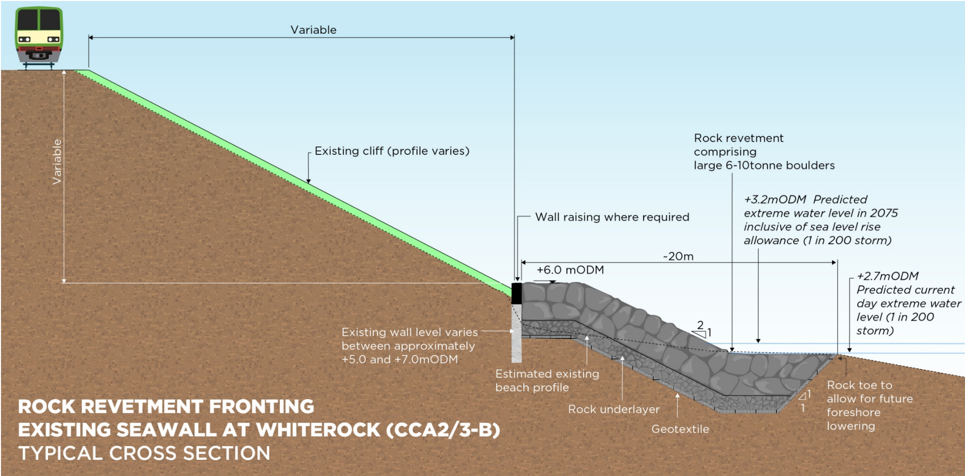
Figure 5-8 CCA2/3 Emerging Preferred Scheme Section at Whiterock
