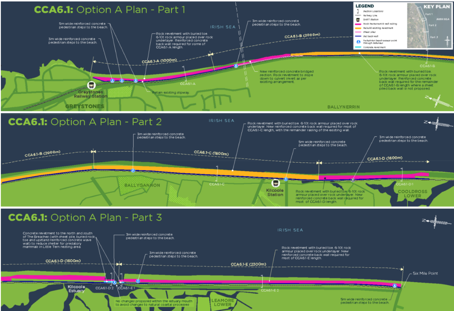
Figure 5-1 CCA6.1 Option A Concept Design Plan
