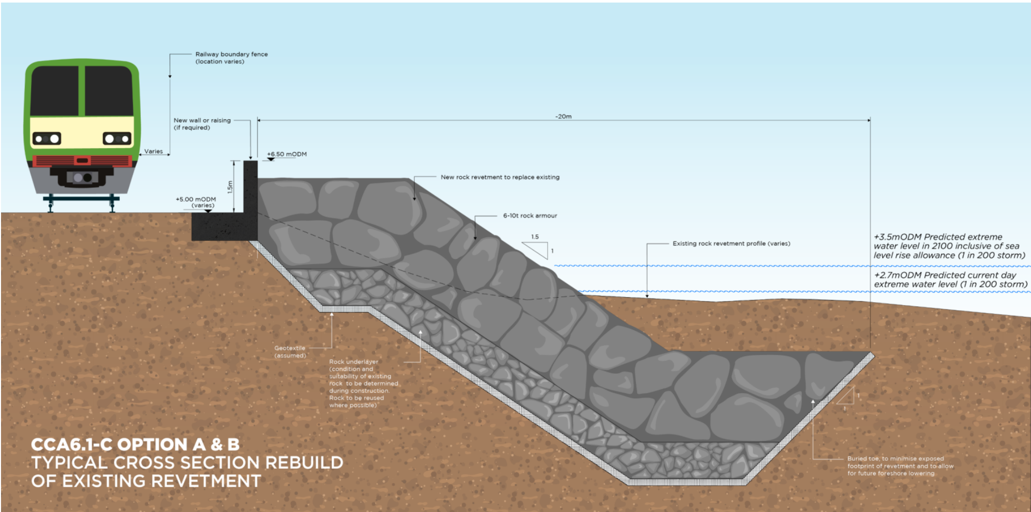
Figure 5-2 CCA6.1-C Option A & B typical cross section
