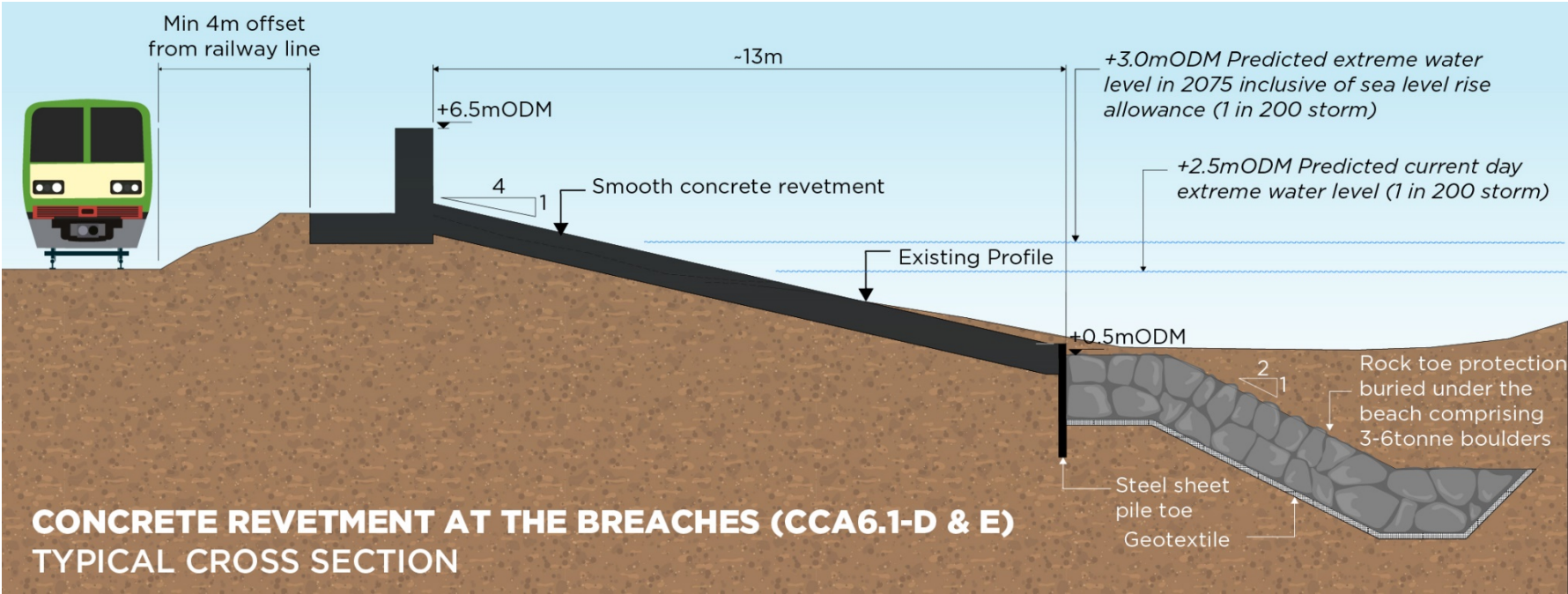
Figure 5-8 CCA6.1 Emerging Preferred Scheme typical section at The Breaches
