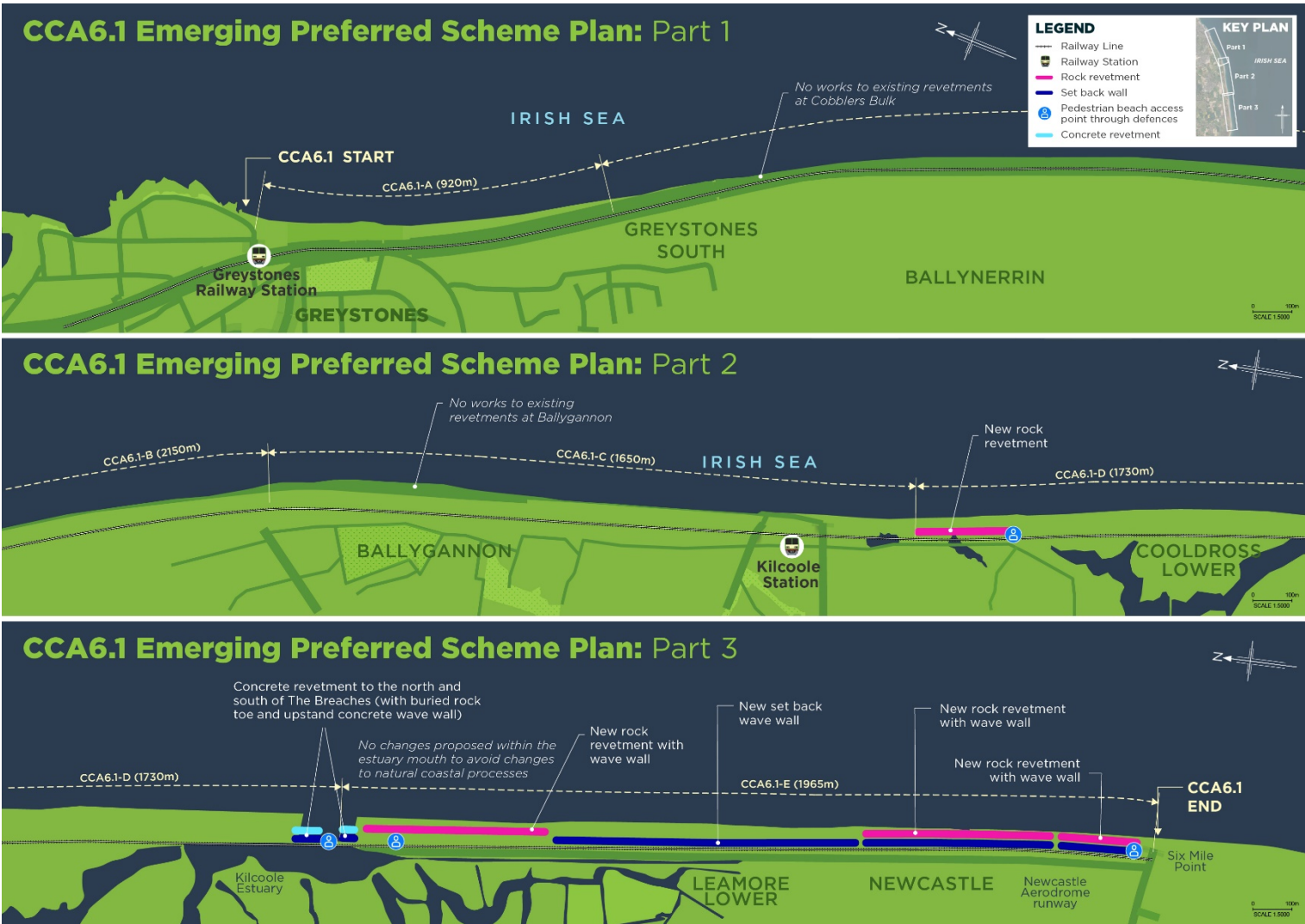
Figure 5-6 CCA6.1 Emerging Preferred Scheme Plan
