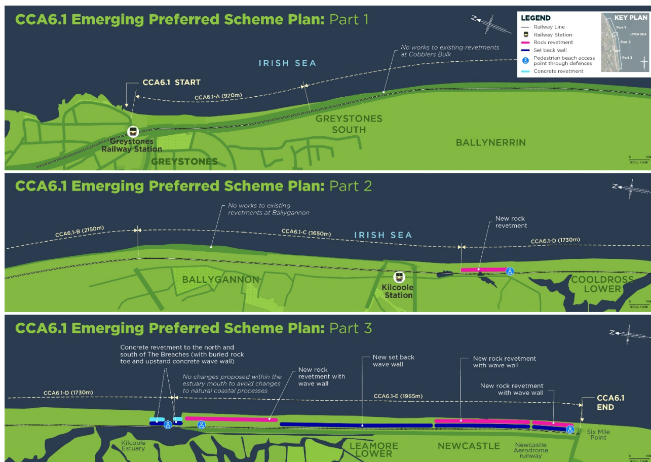
Figure ES: CCA6.1 Emerging Preferred Scheme Plan
