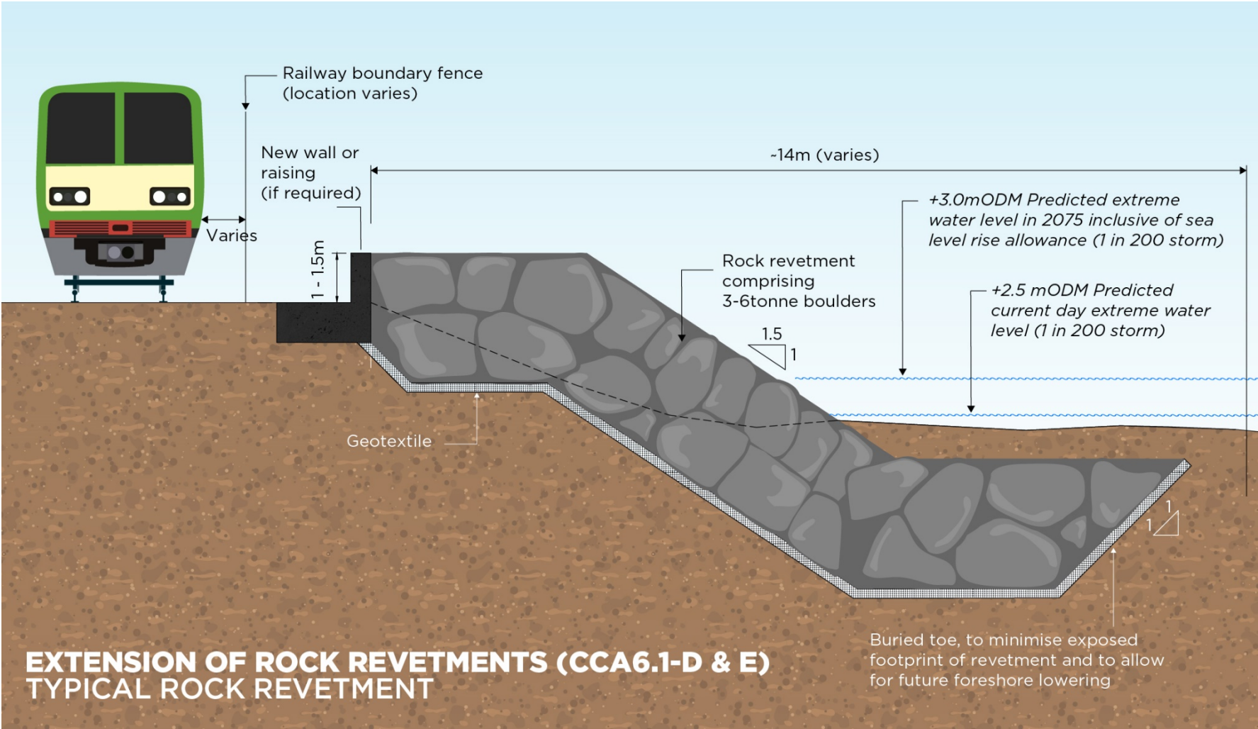
Figure 5-7 CCA6.1 Emerging Preferred Scheme typical section
