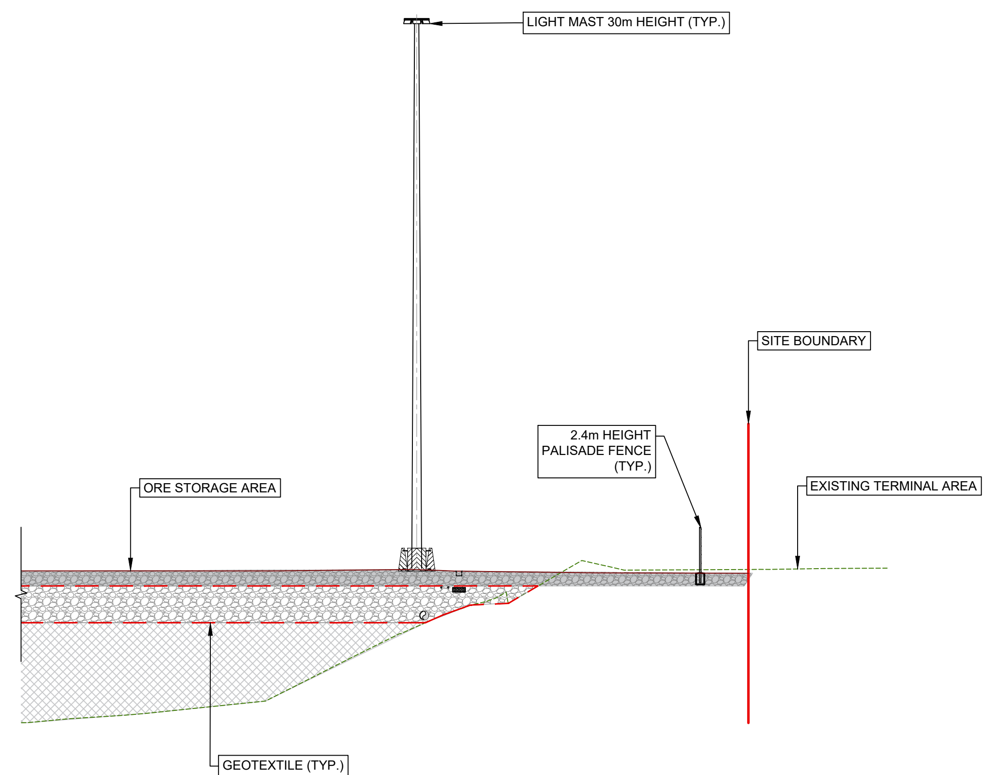
SECTION C-C-VIEW 6 SCALE 1:200
