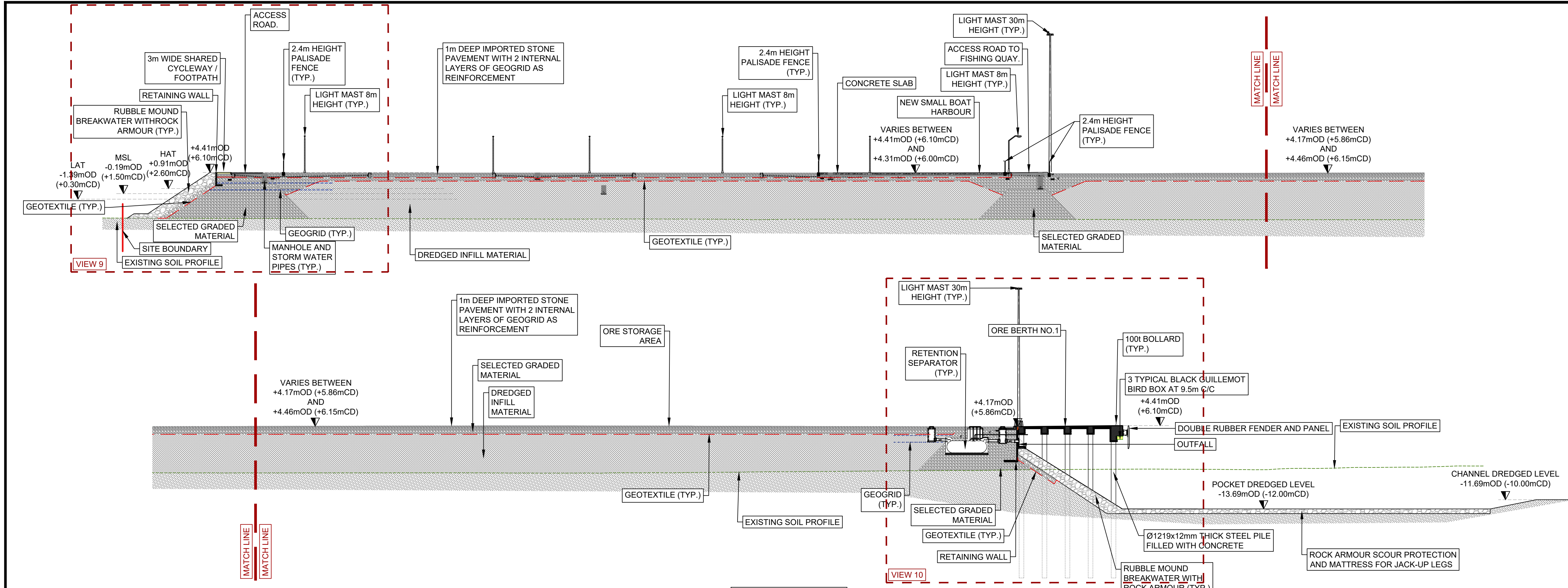
SECTION E-E SCALE 1:500
